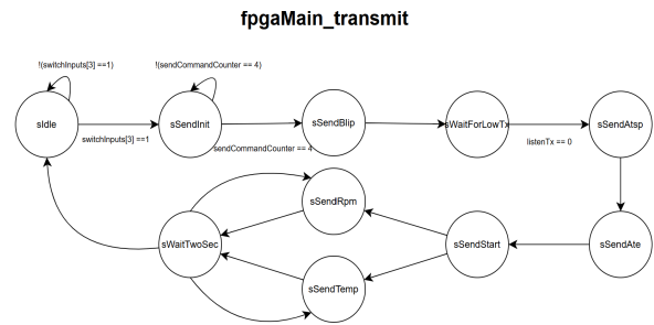
Figure 1.3.9: fpgaMain_transmit FSM
