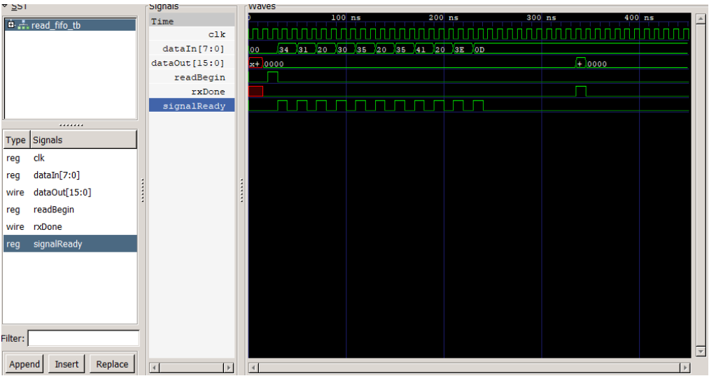
Figure 3.4: read fifo
