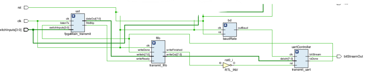
Figure 2.3: Complete UART Write Block Diagram
