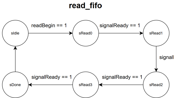
Figure 1.3.5: read_fifo FSM
